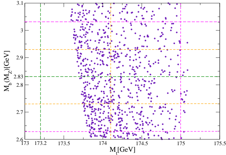
Figure 3: Using the regions of values for K_\tau = Y_\tau^2/g_3^2 and \tan\beta which give experimentally accepted tau mass, this figure shows the resulted points in the (M_t, M_b) phase space. The central value (green dashed lines), as well as the 1 and 2\sigma deviation (orange and magenta lines respectively), for the top and bottom masses is also drawn.
