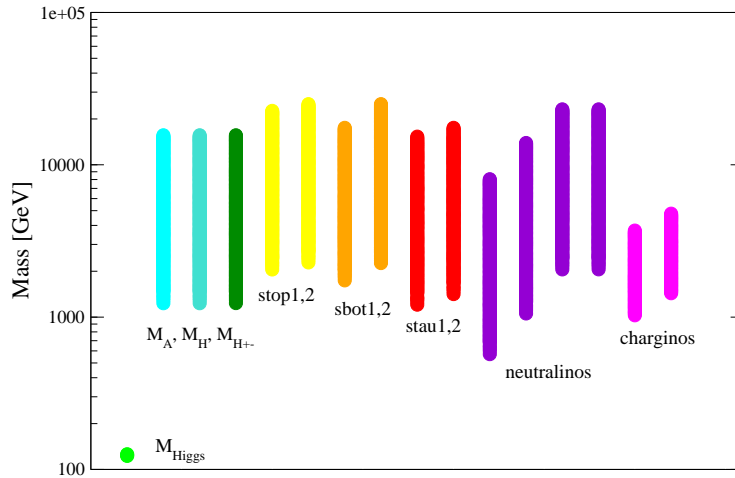
Figure 5: The Higgs mass and s-spectrum for values of M_U \sim 1.3 TeV to \sim 11 TeV.
