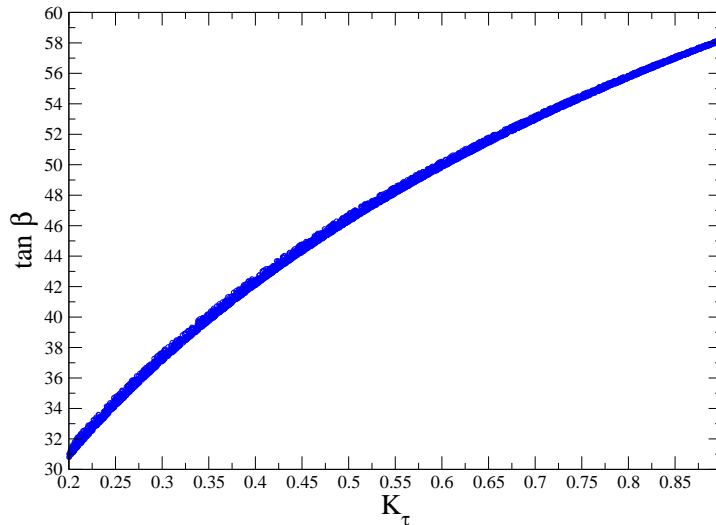
Figure 1: Required values of \tan \beta as a function of K_\tau = Y_\tau^2 / g_3^2 in order to get the experimentally accepted tau mass.
