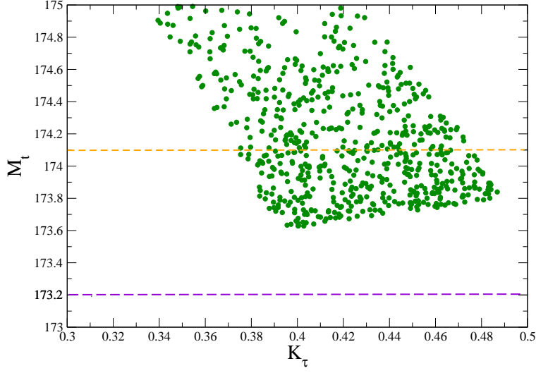
Figure 2: The top mass as a function of K_\tau = Y_\tau^2/g_3^2 , the purple dashed line is the experimental central value and the orange one is the 1\sigma value.
