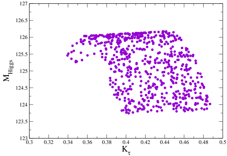
Figure 4: The Higgs mass as a function of K_\tau = Y_\tau^2/g_3^2
